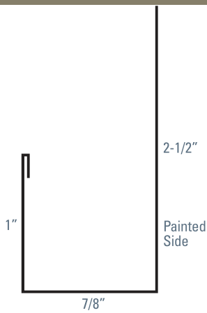
J TRIM
