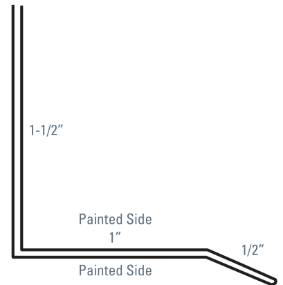
DRIP CAP 1"
