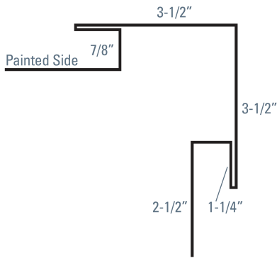
J TRIM
