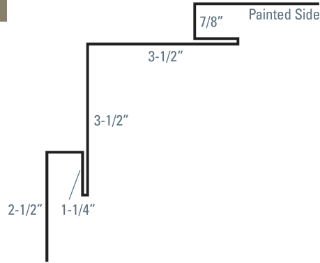
INSIDE CORNER
