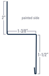
Double Angle
