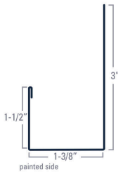
J-Trim
