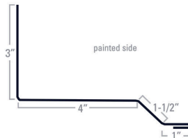
Side Wall
