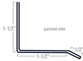
Drip Cap
