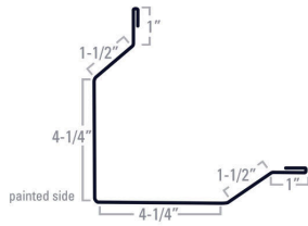
Outside Corner
