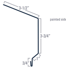
Fascia Eave
