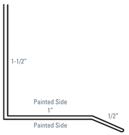
Drip Cap 1"
