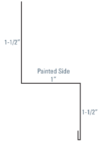
Double Angle
