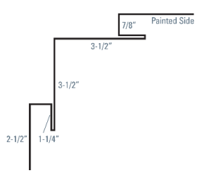
Inside Corner
