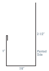
J-Trim
