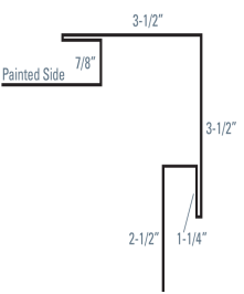
Outside Corner
