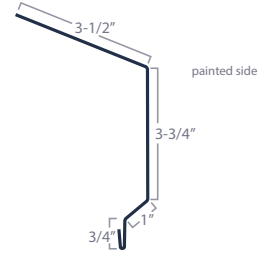
Fascia Eave
