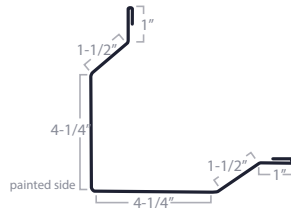
Outside Corner
