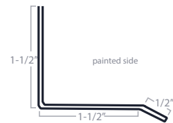
Drip Cap
