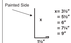
Single Angle
