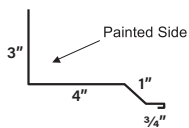
Sidewall
