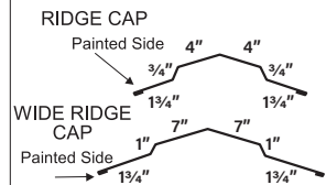
Ridge Caps
