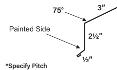
Residential Eave
