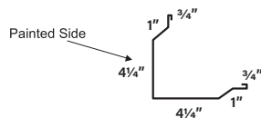
Corner/Rake
