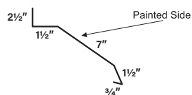
Track Cover
