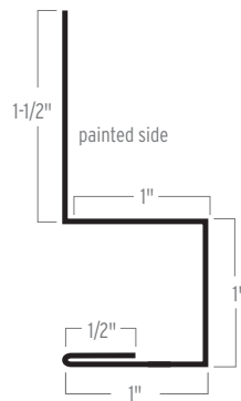
SQUARE BASE TRIM
