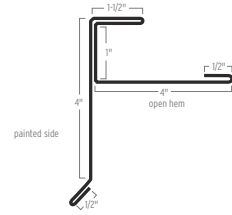
CONCEALED FASTENER RAKE
