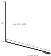
CONCEALED FASTENER DENVER ENDWALL
