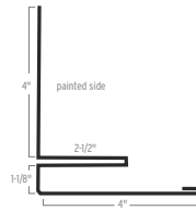
TRIM FIRST CONCEALED FASTENER SIDEWALL
