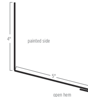
CONCEALED FASTENER ENDWALL
