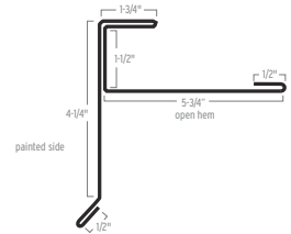
CONCEALED FASTENER RAKE
