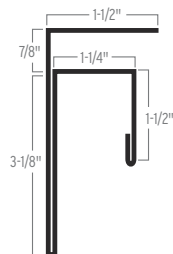
F&J FOR PANEL
