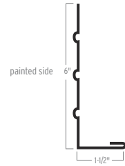
BEADED FASCIA
