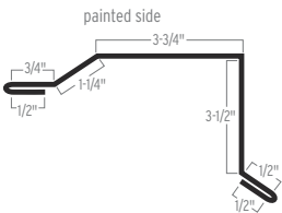
RESIDENTIAL RAKE
