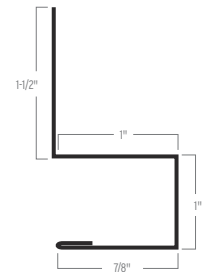
SQUARE BASE TRIM
