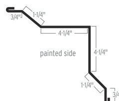
INSIDE CORNER
