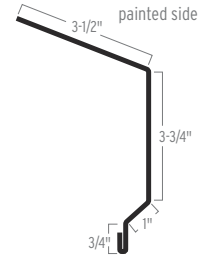
FASCIA EAVE
