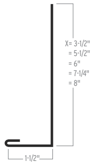
SINGLE ANGLE
