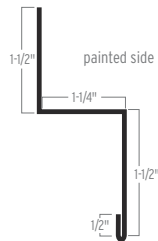
DOUBLE ANGLE
