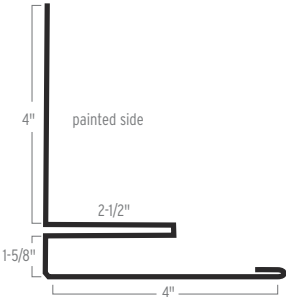
TRIM FIRST CONCEALED FASTENER SIDEWALL
