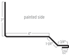
SIDEWALL
