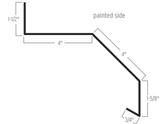
TOP MOUNT TRACK COVER
