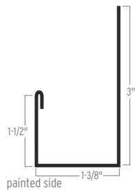
J-TRIM
