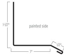
SINGLE BENT DRIP CAP
