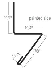
RAT GUARD
