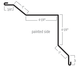
INSIDE CORNER
