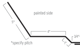
END-WALL
