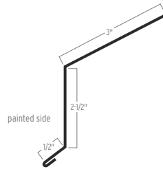
RESIDENTIAL EAVE
