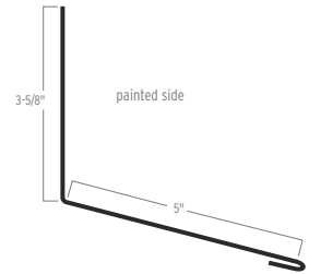
DENVER ENDWALL
