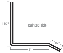
DOUBLE BENT DRIP CAP
