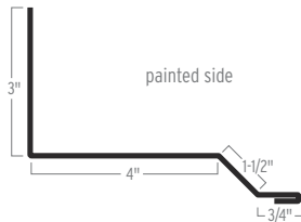
SIDEWALL
