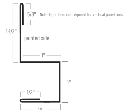
SQUARE BASE TRIM
