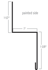
DOUBLE ANGLE
