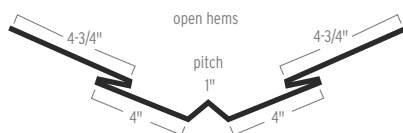
VALLEY TRIM
