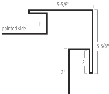
OUTSIDE CORNER
