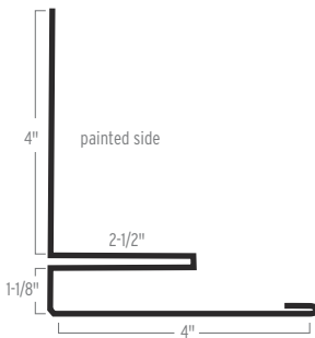
TRIM FIRST CONCEALED FASTENER SIDEWALL
