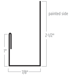
J-TRIM
