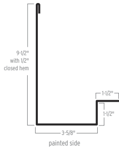
DJ8 WIDE JAMB TRIM
