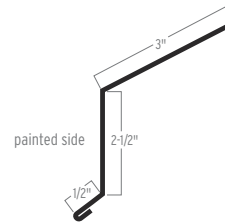
RESIDENTIAL EAVE
