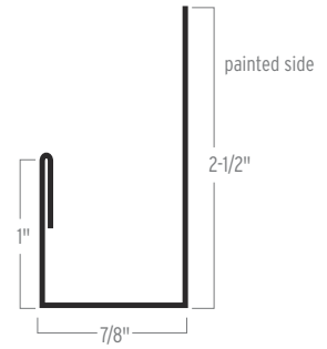
J-TRIM
