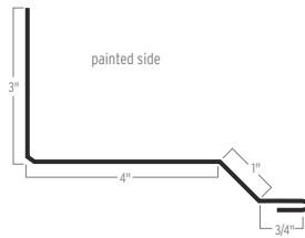
SIDEWALL
