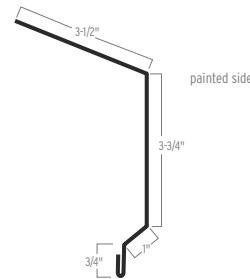
FASCIA EAVE
