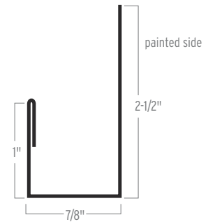
J-TRIM
