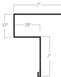
SOFFIT TRIM FOR SOFFIT
