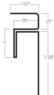
F&J FOR SOFFIT
