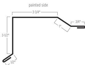
RESIDENTIAL RAKE
