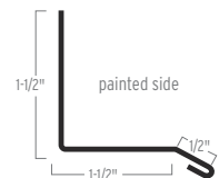
SINGLE BENT DRIP CAP
