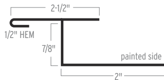
MODERN PLANK SEAM TRIM PART 2
