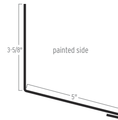
DENVER ENDWALL
