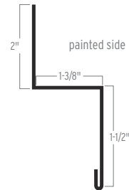
DOUBLE ANGLE
