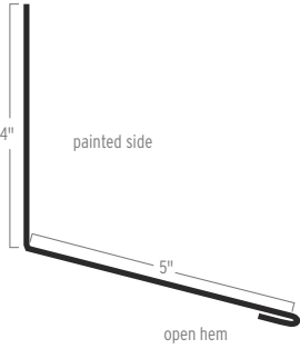
CONCEALED FASTENER DENVER ENDWALL
