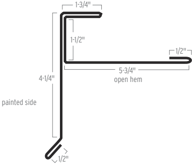
CONCEALED FASTENER RAKE
