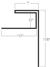
F-TRIM FOR SOFFIT
