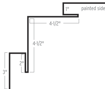
INSIDE CORNER
