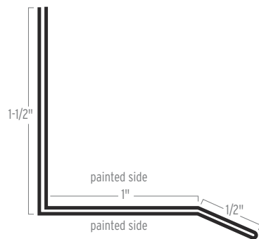
DRIP CAP 1"
