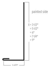
SINGLE ANGLE
