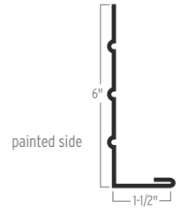
BEADED FASCIA
