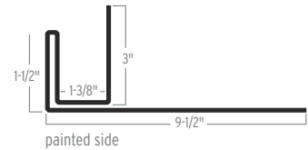
OVERHEAD DOOR TRIM
