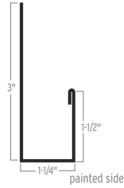
J-TRIM
