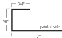
MODERN PLANK SEAM TRIM PART 1
