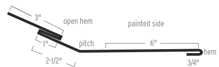
TRANSITION TRIM
