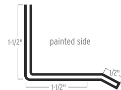
DRIP CAP
