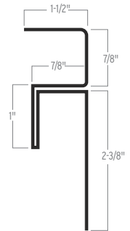
F&J FOR PANEL
