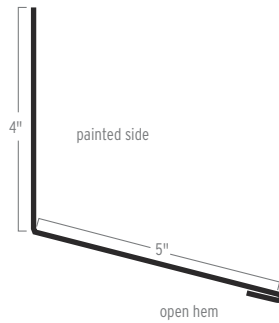
CONCEALED FASTENER ENDWALL
