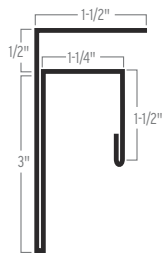
F&J FOR SOFFIT
