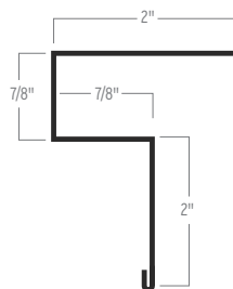
SOFFIT TRIM FOR PANEL
