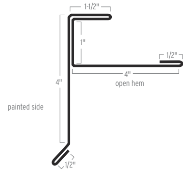
CONCEALED FASTENER RAKE
