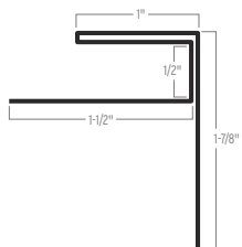
F TRIM FOR SOFFIT
