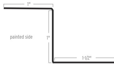
SOLID & VENTED Z TRIM
