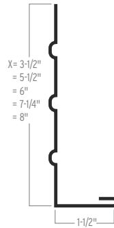
BEADED FASCIA
