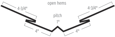
VALLEY TRIM
