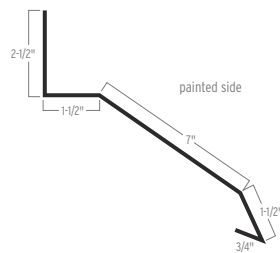
FACE MOUNT TRACK COVER
