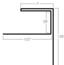
F TRIM FOR PANEL
