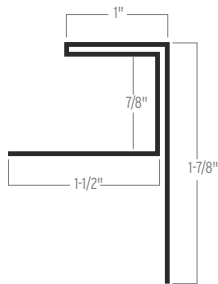
F-TRIM FOR PANEL
