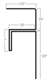
F&J FOR PANEL
