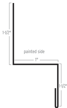
DOUBLE ANGLE
