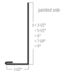
SINGLE ANGLE
