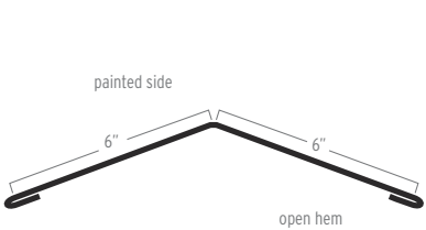
CONCEALED FASTENER RIDGE
