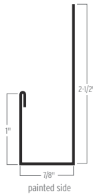
J-TRIM
